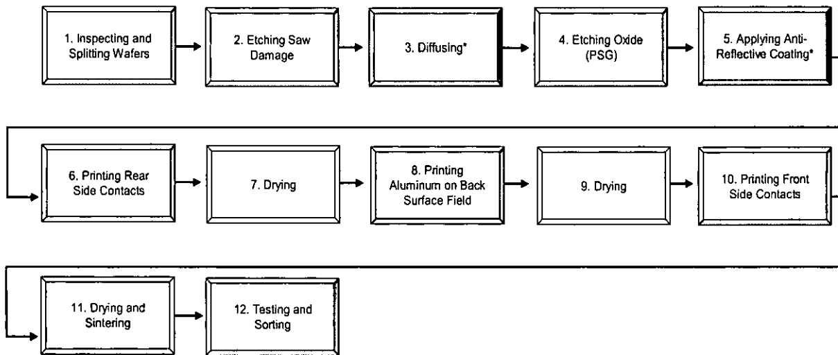
Solar Cell Manufacturing Process Flow Chart
